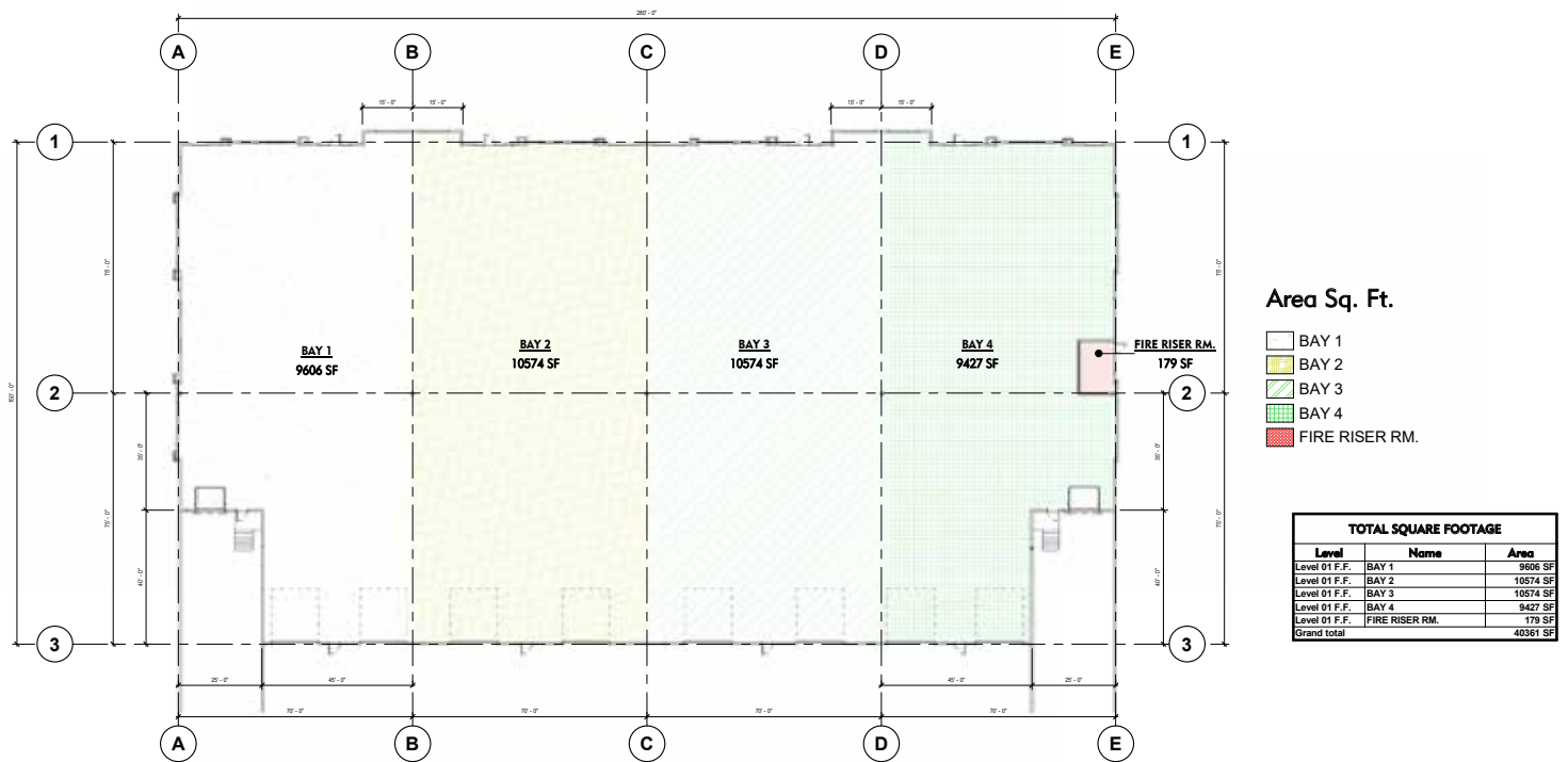
Main Floor Area Plan By Bays 3/64" = 1'-0"
